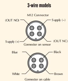
Connectors
