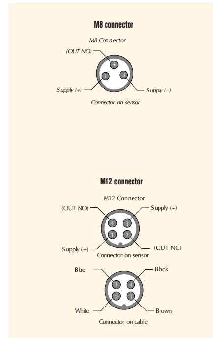
Connectors
