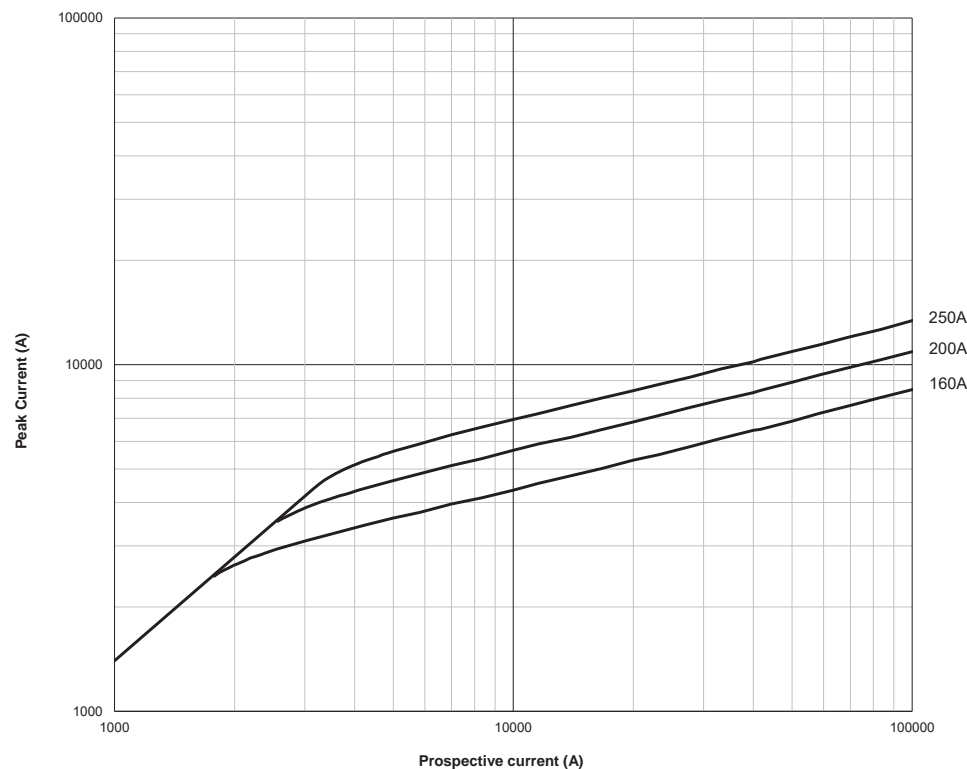
Cut-off peak current curve - Size 2, 160 A to 250 A
